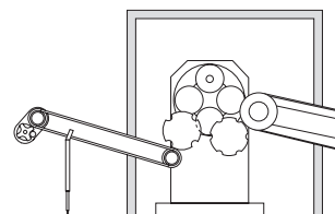
Four heads trimming machine Production speed up to 300 ppm
