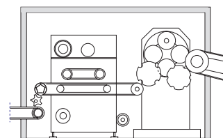
Four cutting heads Tape brushing device
