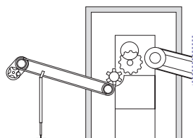
Single head trimming machine Production speed up to 170 ppm
