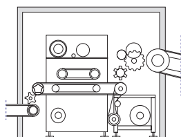
Single cutting head Tape brushing device
